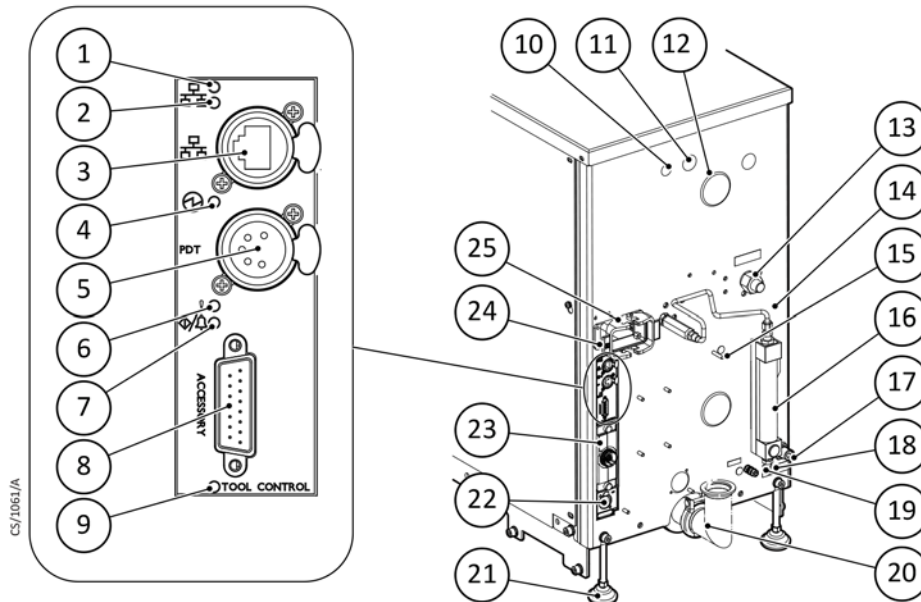
Figure 3 - The controls/connectors on the rear of the pump (system with rear exhaust and castors/levelling feet fitted)
